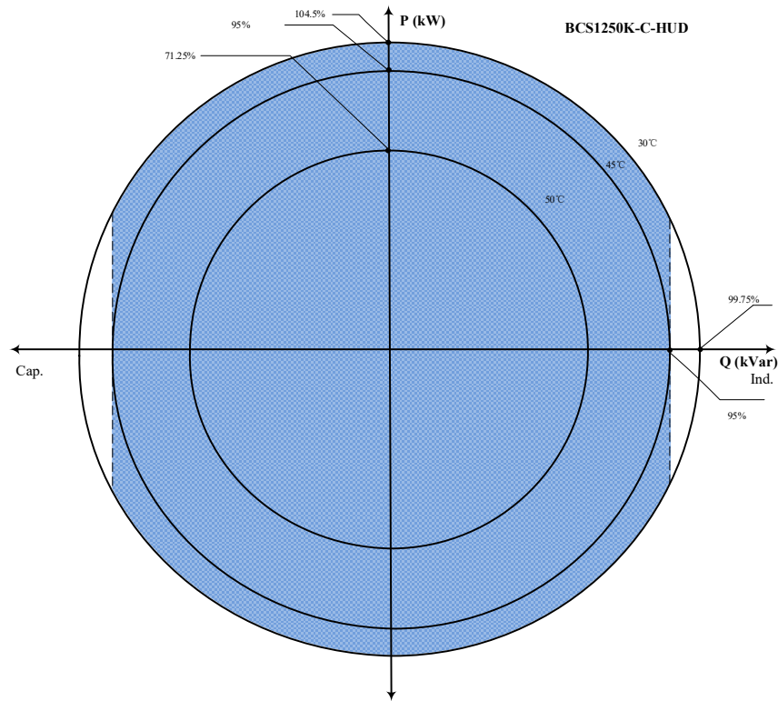
0.95 Rated grid voltage P-Q Curve(Different temperature)
