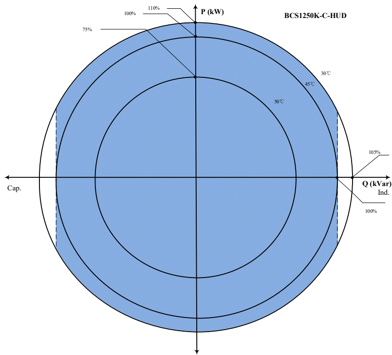
Rated grid voltage P-Q Curve(Different temperature)
