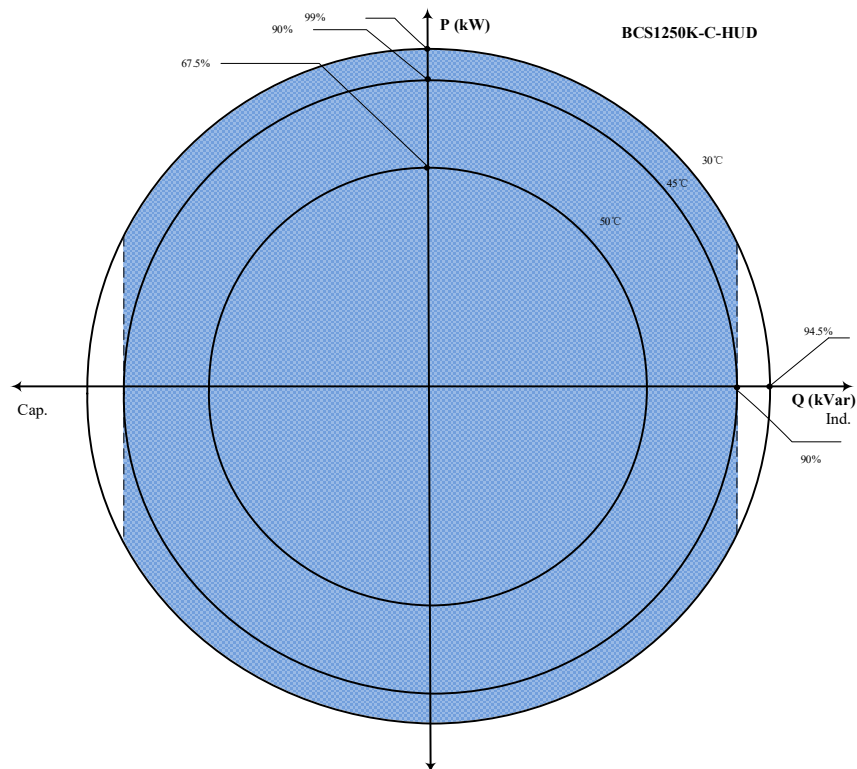
0.9 Rated grid voltage P-Q Curve(Different temperature)
